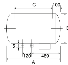
Horizontal 150 - 200 L
